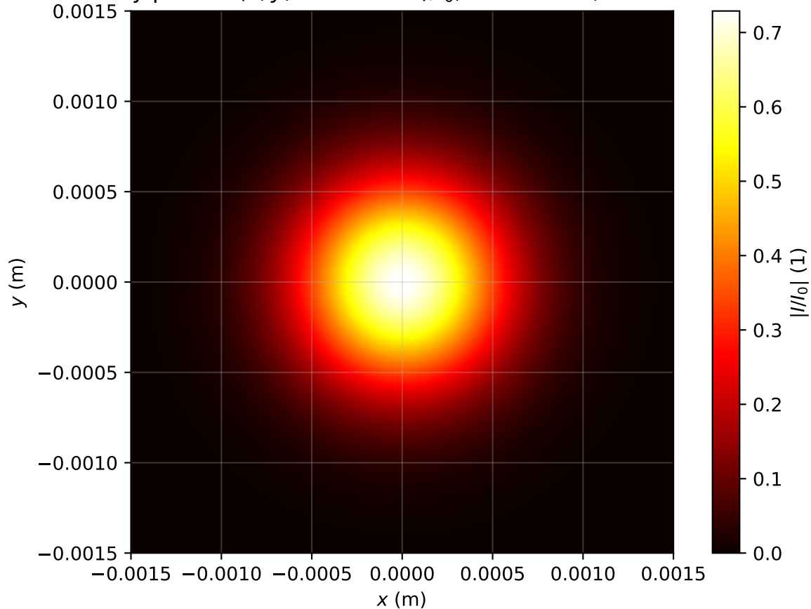
Intensity profile I(x, y, z = 1.353m)/I_0 , Pin=0.1Pcr, artificial time
